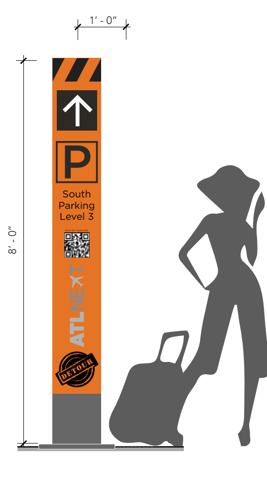
4 FINISH - ELEVATION SIDE A SCALE: 1/2" = 1' - 0"
