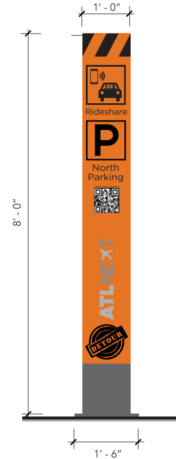
7 FINISH - ELEVATION SIDE B SCALE: 1/2" = 1' - 0"
