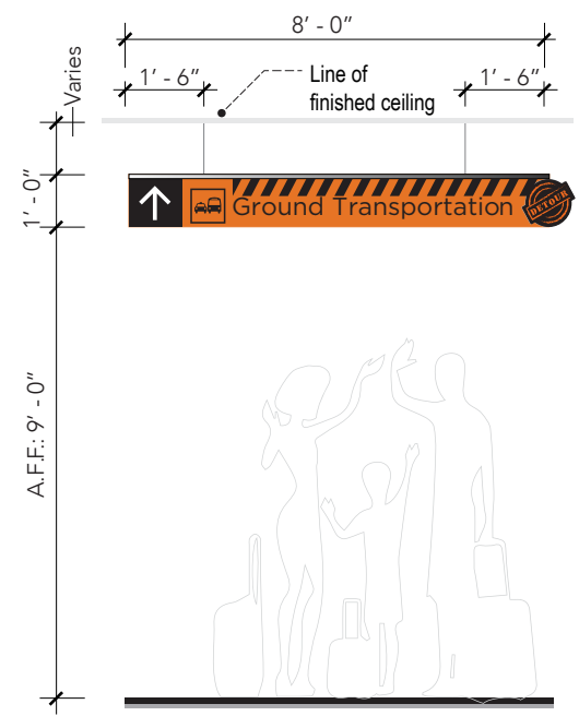
6 ELEVATION (SUSPENDED) SCALE: 1/2" = 1' - 0"
