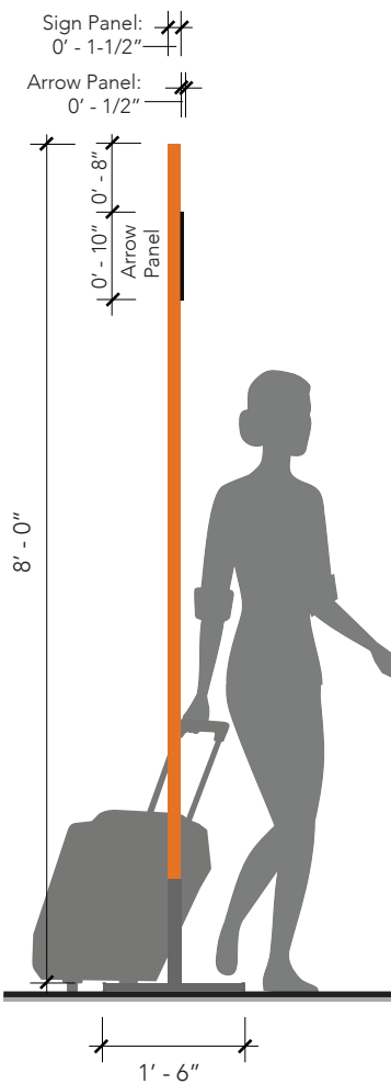
5 FINISH - PROFILE SCALE: 1/2" = 1' - 0"
