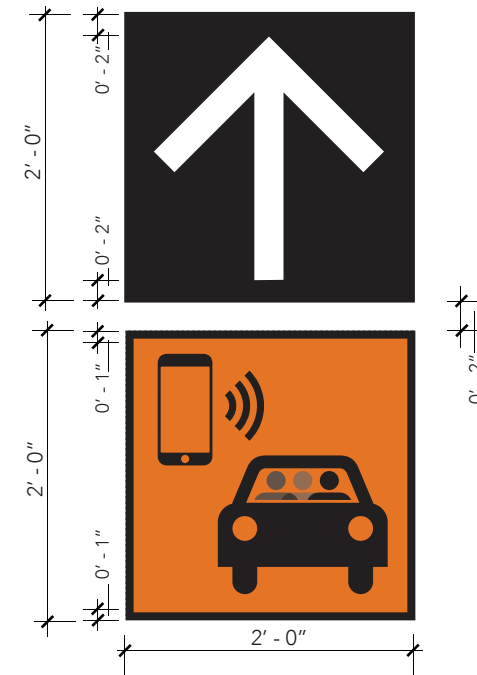
4 FINISH SCALE: 3/4" = 1' - 0"
